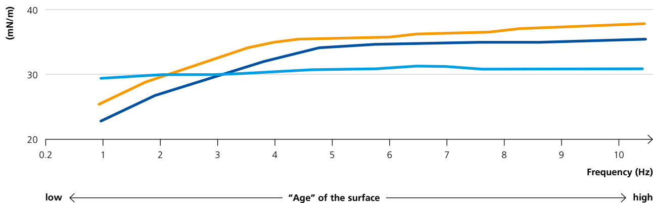
Insufficient wetting without surface additive
